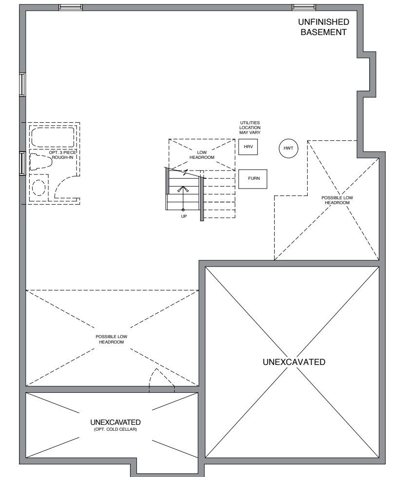
BASEMENT FLOOR ELEVATION A
